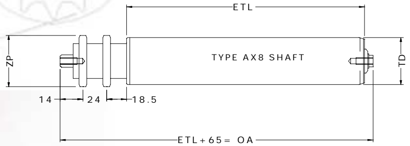
Fixed drive rollers with Female Thread (AX8) Fixing
