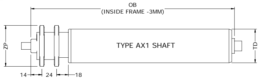
Fixed drive rollers with Sprung Shaft (AX1) Fixing
