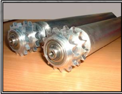
Fixed drive rollers with Female Thread (AX8) Fixing
